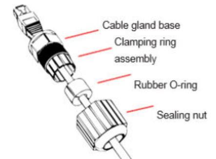
FIGURE 3 RJ-45 Cable and Cable Gland Assembly
