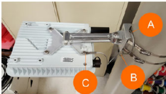
FIGURE 13 Attaching the Security Cable
